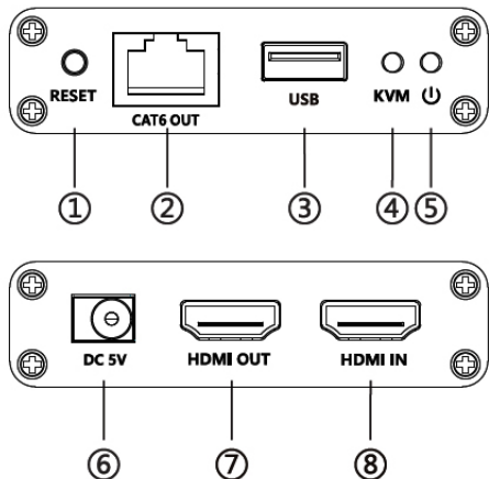
Figure 1: Transmitter (TX)
