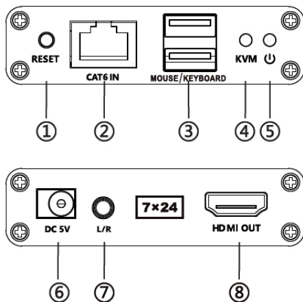
Figure 2: Receiver (RX)
