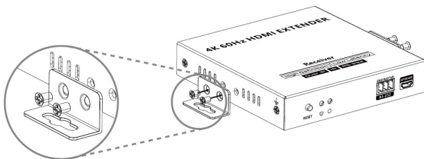
Figure 3: Surface Mount
