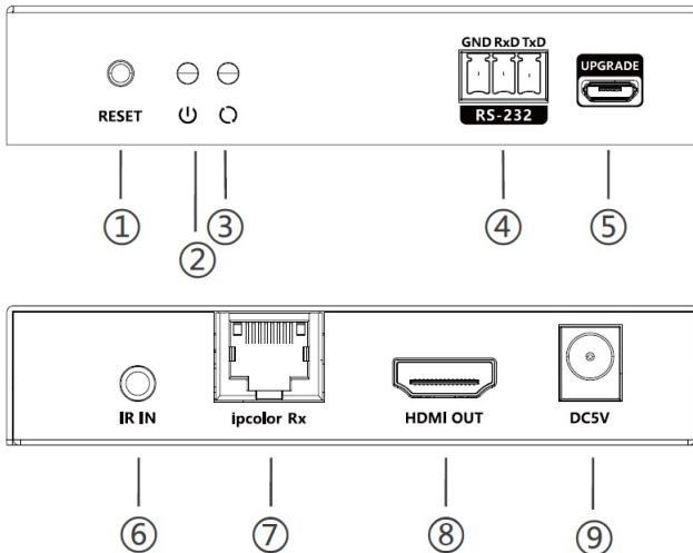
Figure 2: Receiver (RX) Front and Rear Panel Layout
