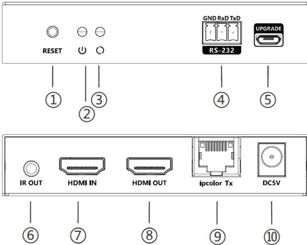
Figure 1: Transmitter (TX) Front and Rear Panel Layout
