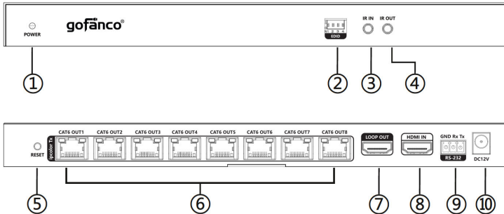
Figure 1: Transmitter Layout
