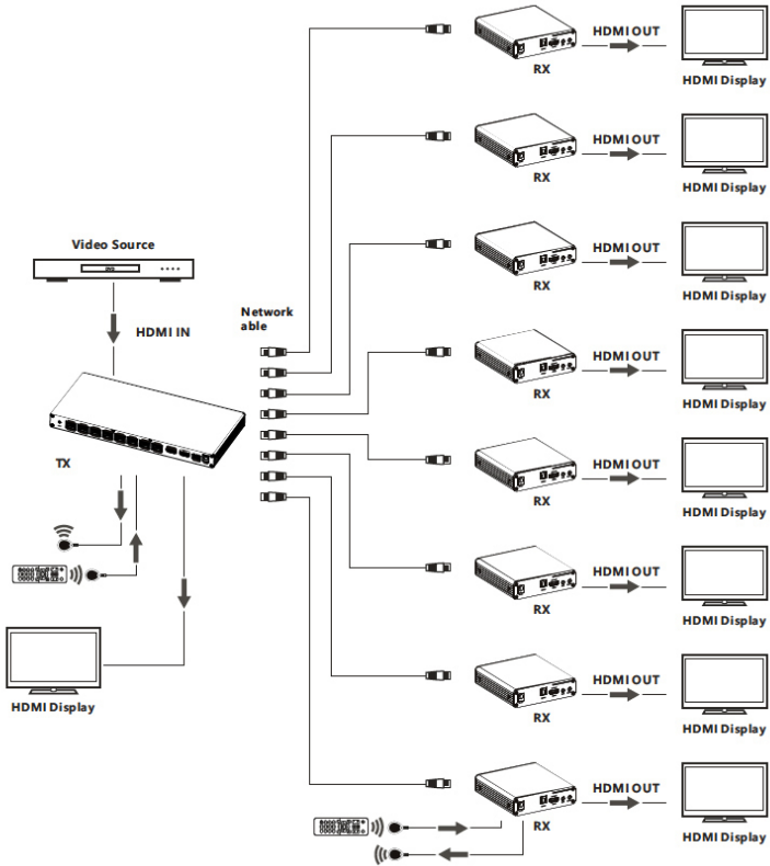
Figure 4: Application Diagram
