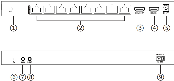
Figure 1: Transmitter Layout
