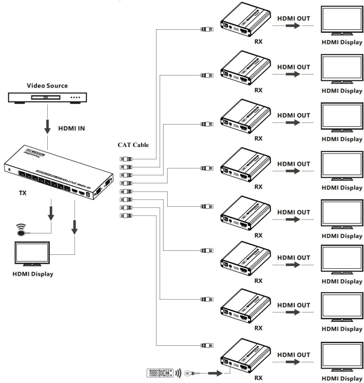
Figure 4: Application Diagram
