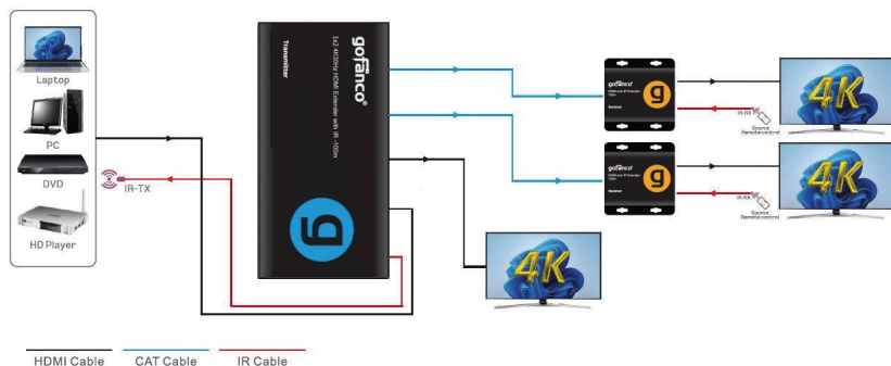
Figure 3: Direct Connection Diagram
