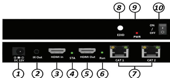
Figure 1: Transmitter (TX)
