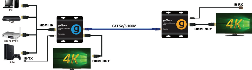
Figure 3: Connection Diagram
